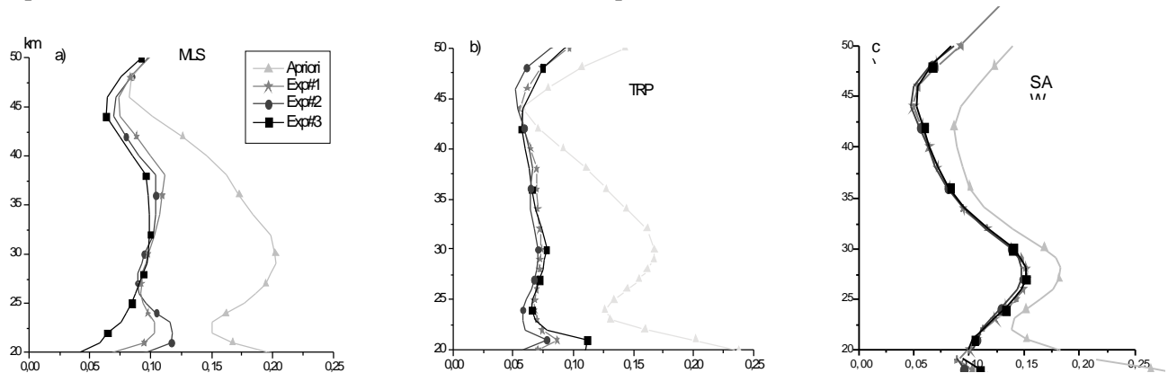
Fig.1 Ozone profile retrieval error statistics in Experiments #1-3
