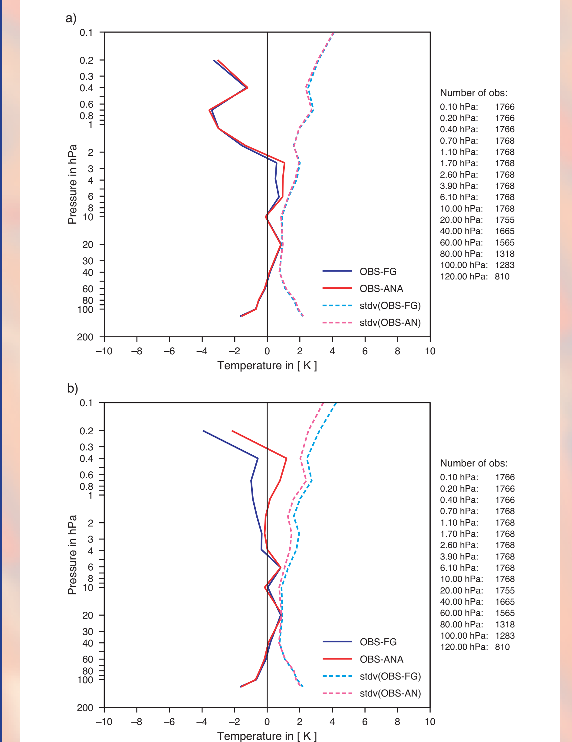
Figure 5 Departure statistics for ESA's MIPAS temperature retrievals (bias-solid; standard deviation-dotted) for the region 65–20°N, without (a) and with (b) MIPAS radiance assimilation.
