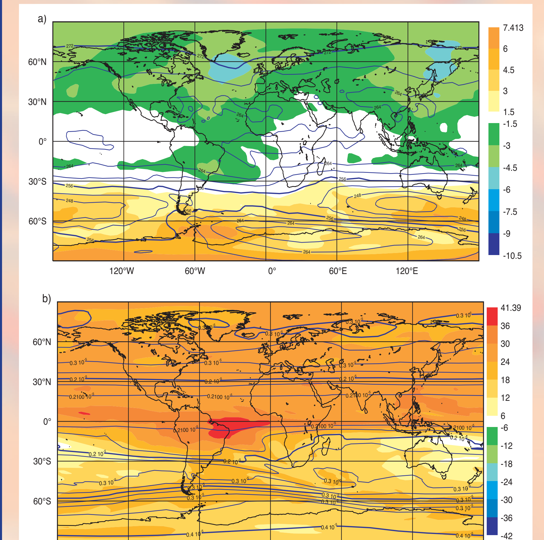
Figure 4 a) Difference in mean temperature analyses [K] at 1 hPa between the experiment with and the one without MIPAS radiance assimilation. b) Relative difference in the mean humidity analyses [%] at 10 hPa between the experiment with and the one without MIPAS radiance assimilation.
