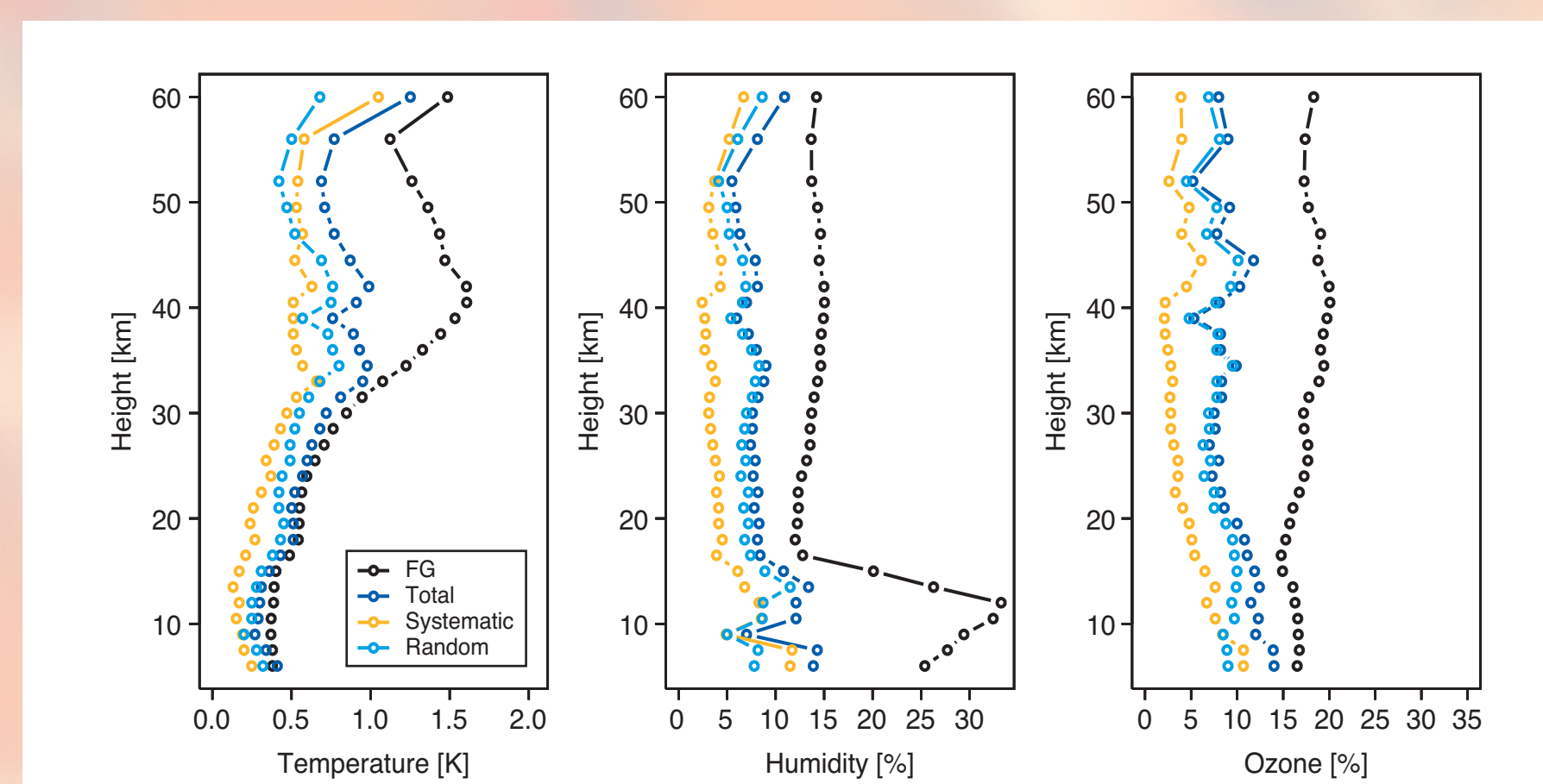
Figure 2 Theoretical reduction of analysis error that can be achieved with the selected MIPAS data. Black is the ECMWF background error; light blue the retrieval error expected if only MIPAS instrument noise and the background error are taken into account; orange is the estimate of errors introduced through the forward model (e.g., spectroscopic uncertainty, fixed climatology for certain gases, etc); blue the expected total retrieval error.
