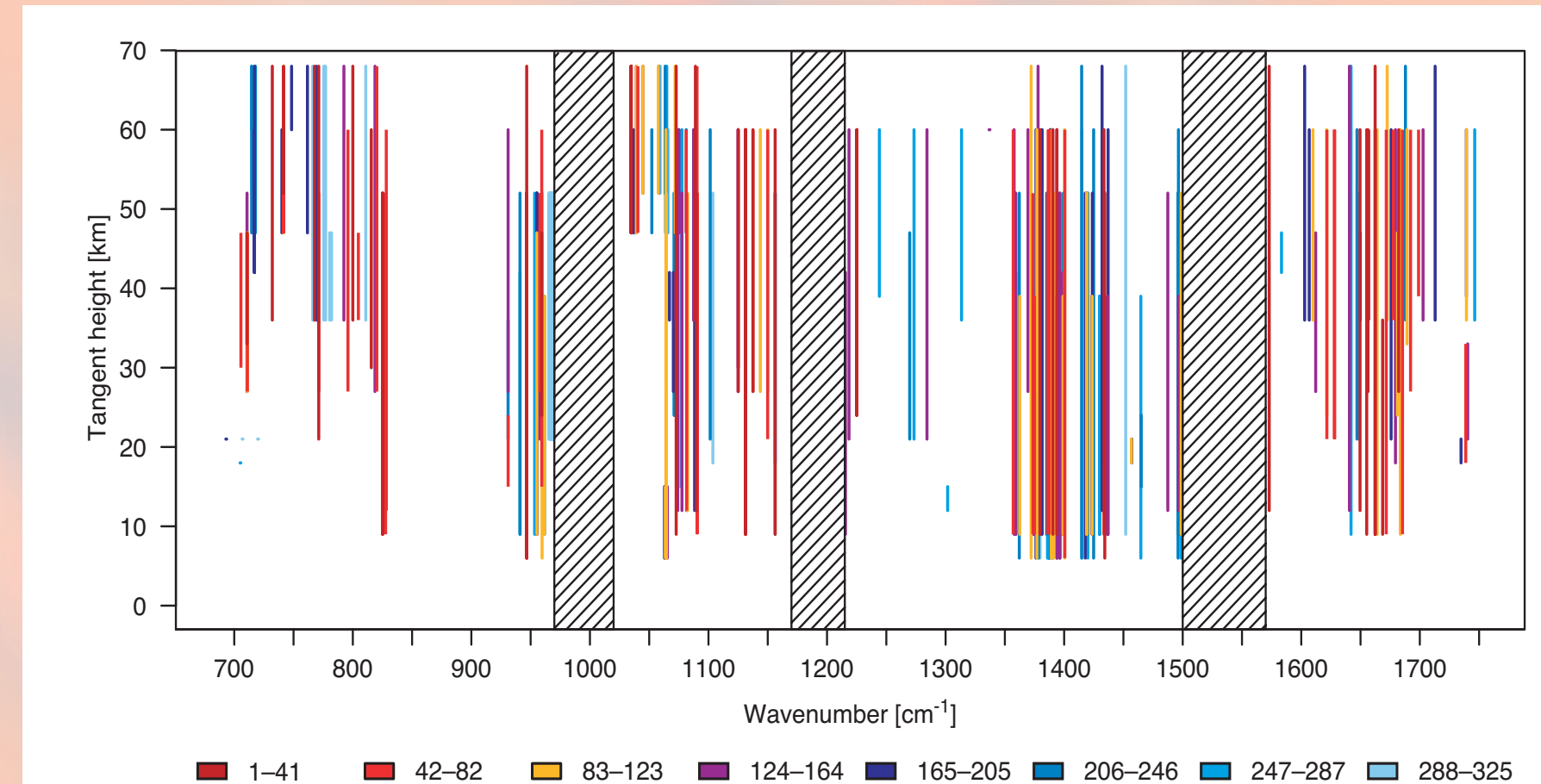
Figure 1 Location of the selected MIPAS channels and tangent heights. Colour coding gives the ranking in the selection.
