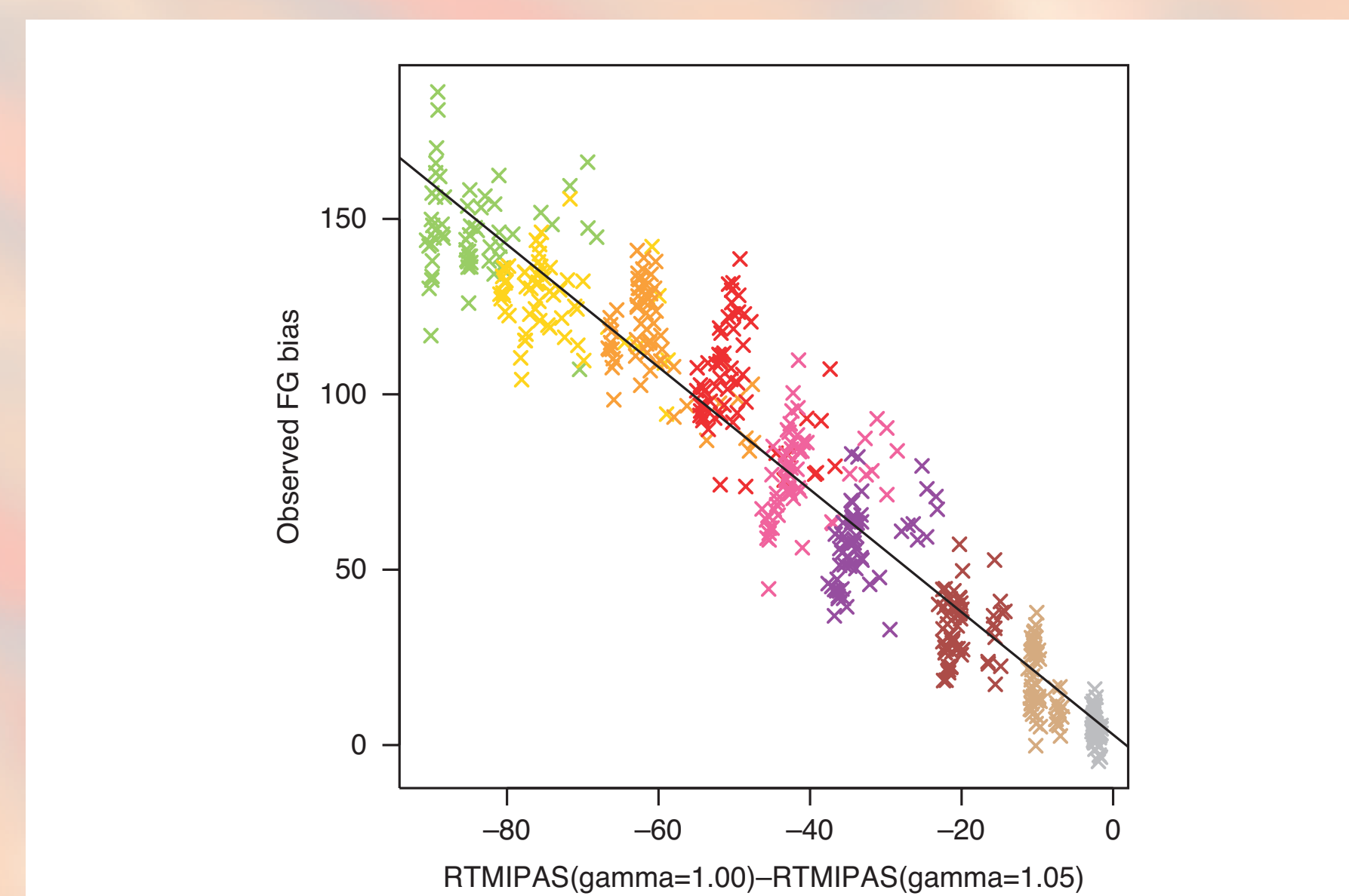
Figure 3 FG bias (from 30 x 20° longitude/latitude boxes) vs. the signature of a 5% perturbation in gamma for a MIPAS temperature channel (both in nW/(cm² sr cm⁻¹)). Colour coding shows tangent height bands with grey for 60 km and green for 27 km.
