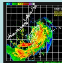
Fig 4 radar echo map at 18 UTC 1 July
