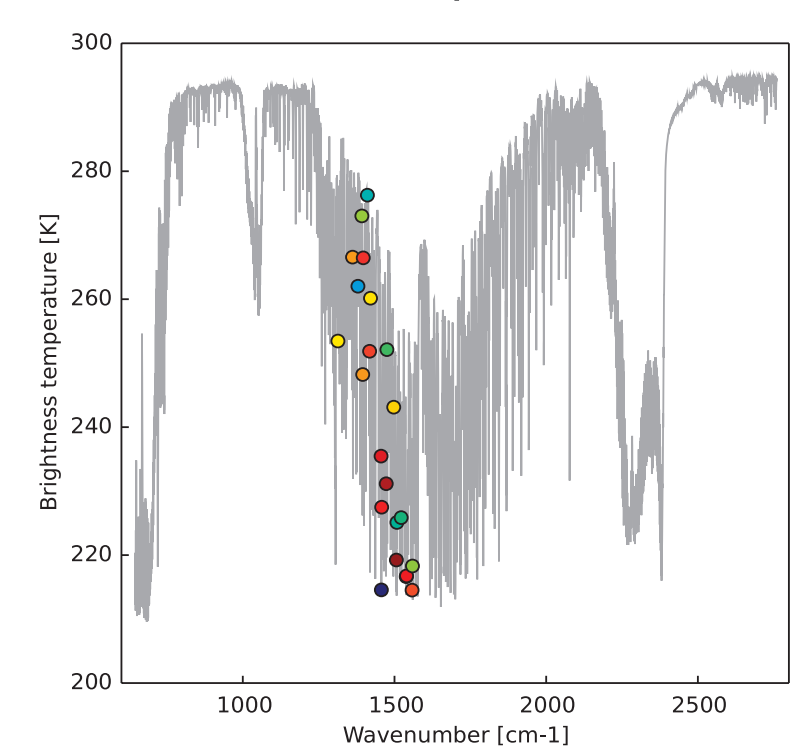
Figure 5 Spectral locations (indicated by coloured circles) of a set of 22 humidity-sensitive IASI channels as selected using the iterative, non-sequential channel selection procedure described in this work. The colour scale denotes the ranking value q_i taken by each selected channel (see text).
