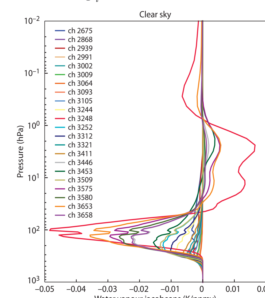
Figure 6 Humidity jacobians of the 22 selected channels
