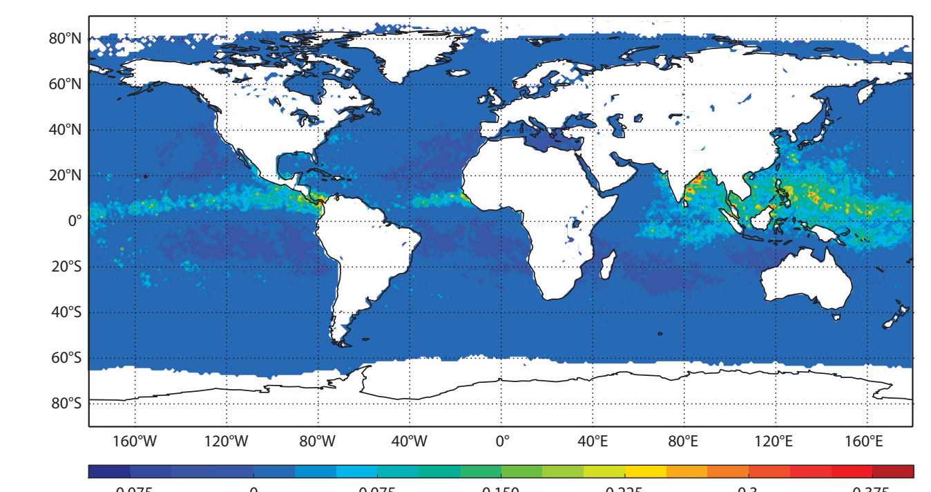
Figure 2 Monthly-mean difference between predicted radiance at IASI channel 3576 (1538.75 cm -1 ) when using the multi-column cloud model and that when using the single-column model, at 1 x 1 deg resolution.
