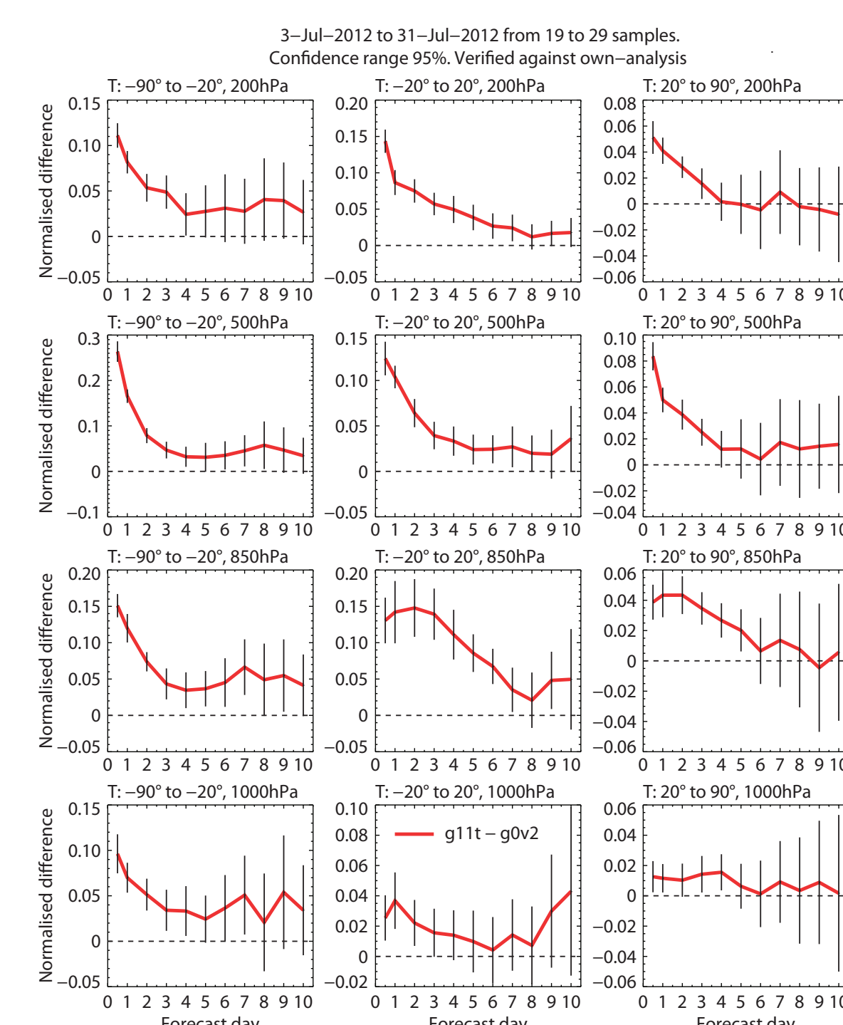
Figure 3 Normalized root-mean-square temperature forecast error difference between experiment with 10 all-sky IASI water vapour channels and experiment with same channels only assimilated in clear sky.
