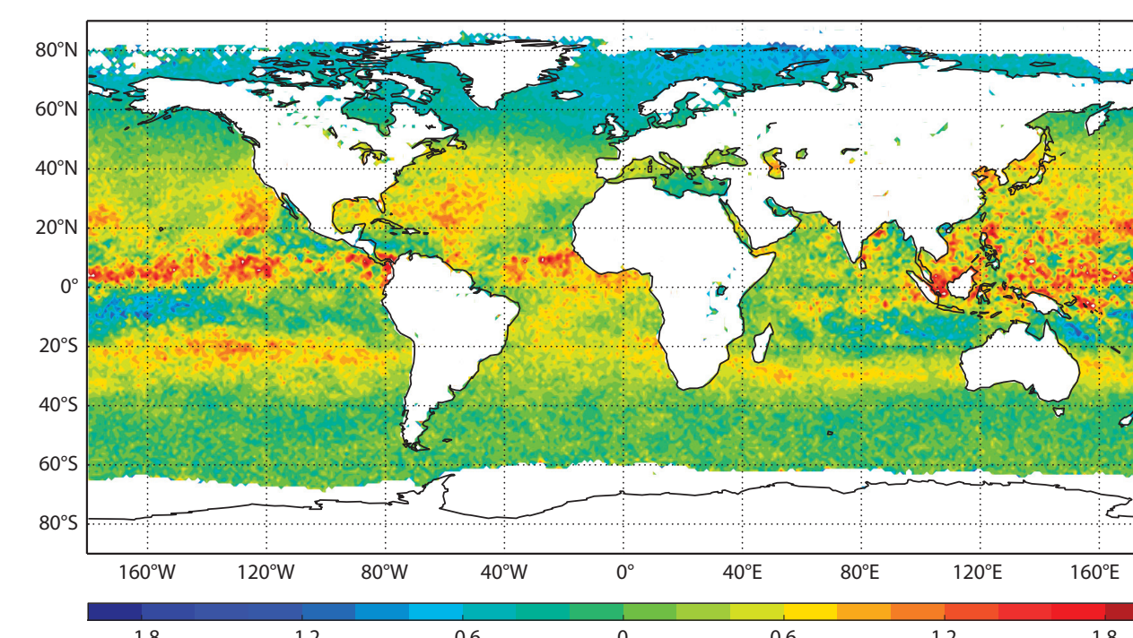
Figure 1 Monthly-mean innovation for IASI channel 3576 (1538.75 cm -1 ) at 1 x 1 deg resolution when cloud radiative effects are simulated using the single-column cloud model.
