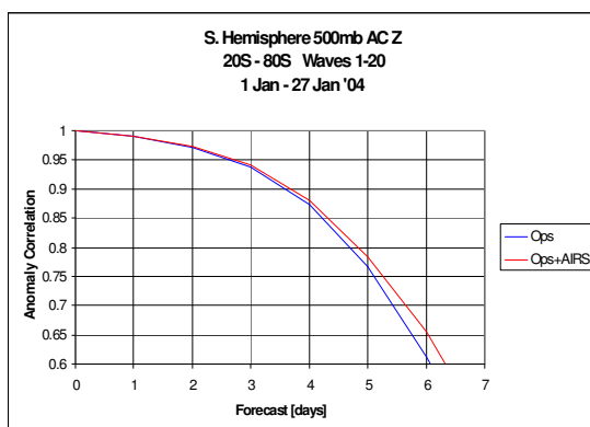
Figure 1 : The impact of AIRS data on GFS forecasts at 500hPa (20°S - 80°S), 1 – 27 January 2004; the pink (blue) curve shows the AC with (without) AIRS data.
