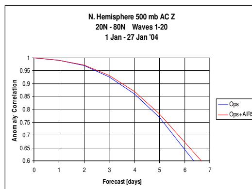
Figure 2 : The impact of AIRS data on GFS forecasts at 500hPa (20°N - 80°N), 1 – 27 January 2004; the pink (blue) curve shows the AC with (without) AIRS data.
