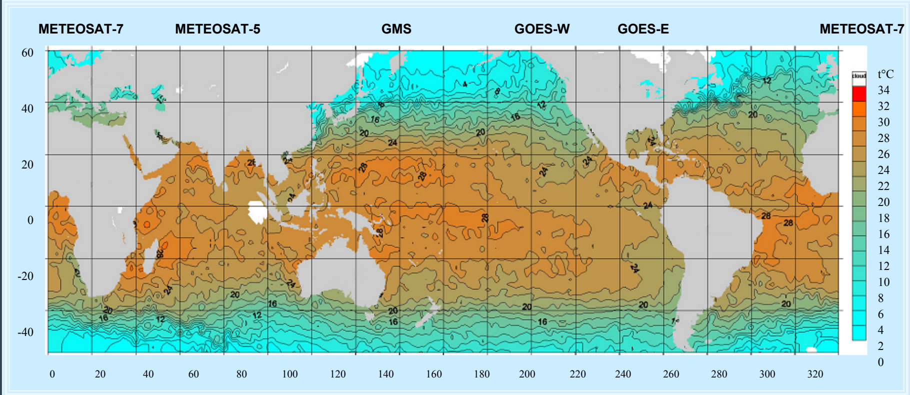
SST MAP COMPOSED FROM METEOSAT, GOES, GMS DATA
