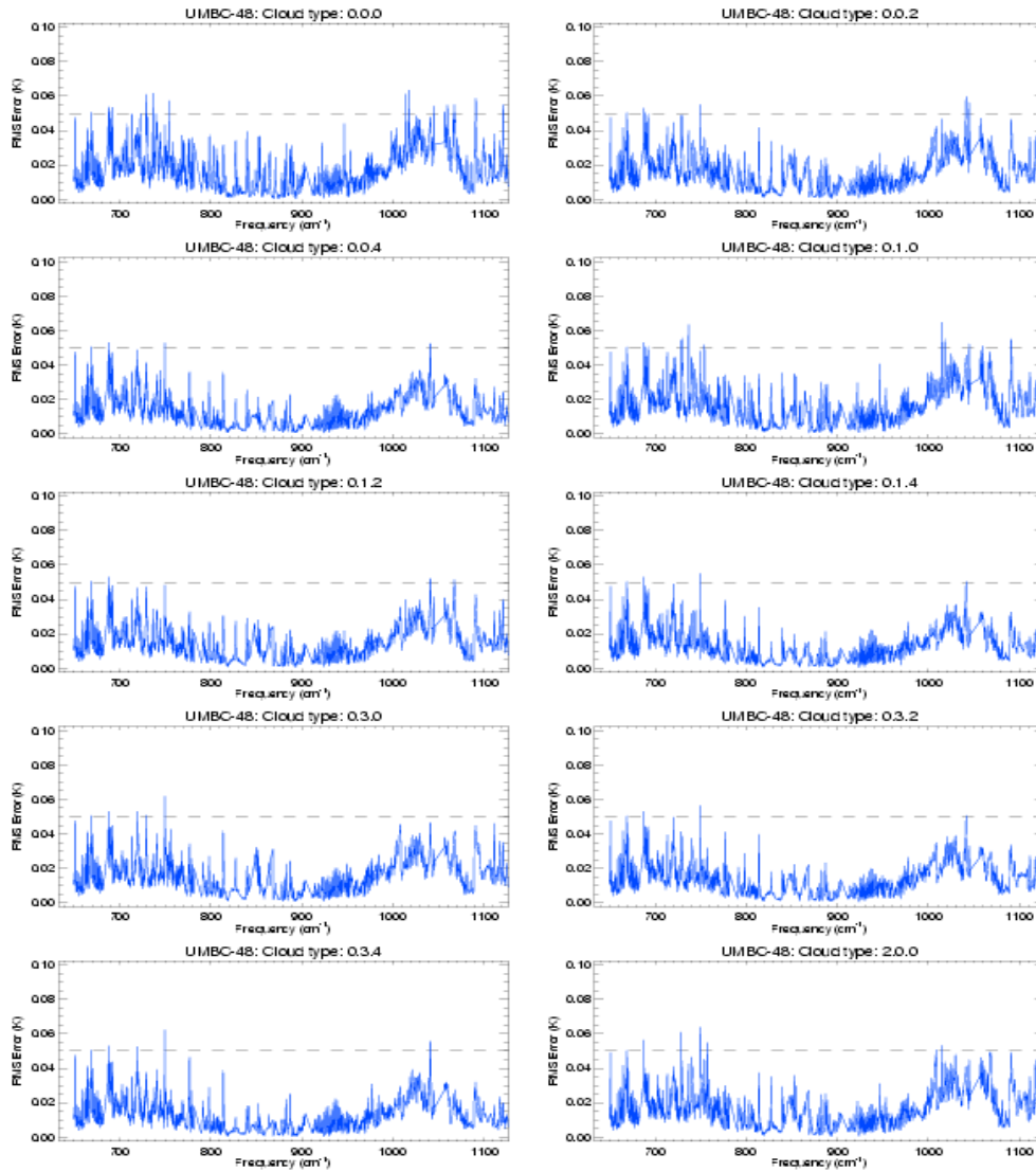
Fig. 4: OSS model accuracy in multi-layer cloudy (purely absorbing case) atmospheres. The upper left plot represent the rms errors in the clear-sky based on 48 profiles from the UMBC standard data set. The remaining plots correspond to different ranges of cloud optical depth in 3 atmospheric layers (low, medium, high). The range of optical depth (OD) corresponding to each layer is indicated by the 3 indices at the top of each plot, the lower layer being represented by the 1 st index. The code used is: 0 = clear, 1= OD < 0.5, 2= OD <1, 3= OD < 2, and 4= OD > 2.
