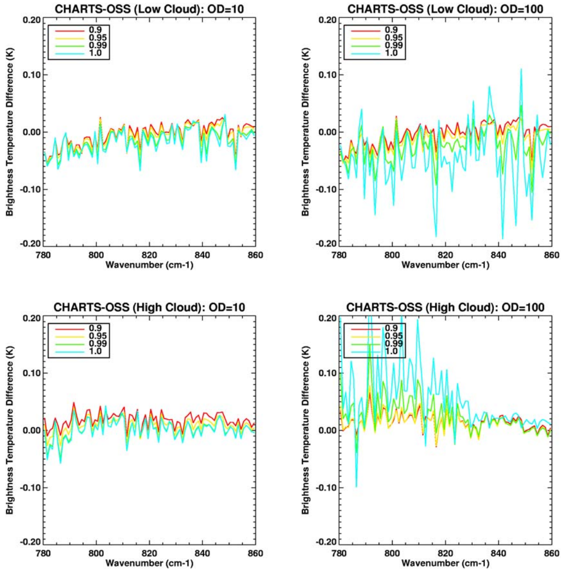
Fig. 1: OSS modeling errors for UMBC profile #1 (Nadir viewing) with low (top pressure = 800mb) and high (top pressure = 150mb) clouds. The results shown in this figure correspond to cloud optical depths of 10 (left) and 100 (right) and single scatter albedos ranging from 0.9 to 1. Clear-sky training was used.
