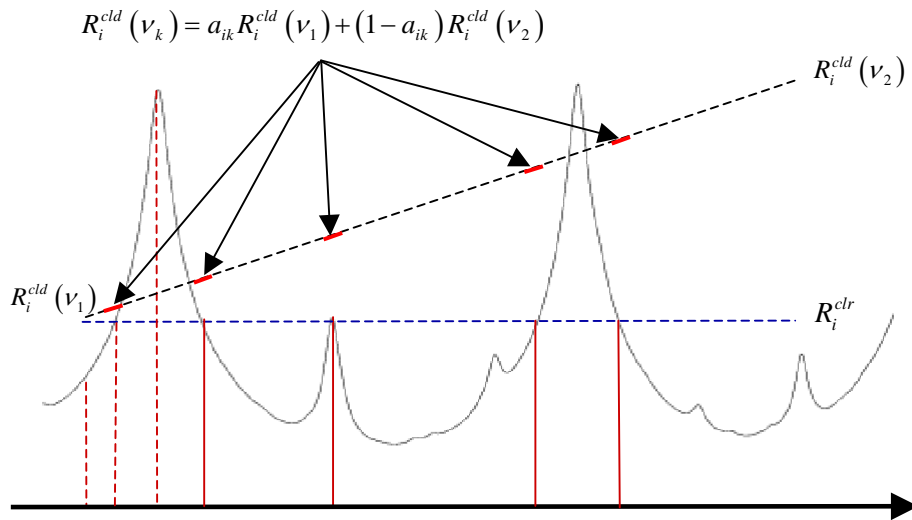
Fig. 3: Example of clear-sky (1 st step) node selection (dashed lines) for an arbitrary spectral domain encompassing a single broadband channel or multiple high-resolution channels. The 4 other spectral sub-intervals represented by the node i=2 are indicated by the solid vertical lines. Clear sky radiances are the same in all the 5 sub-intervals. The impact of clouds on the radiances for this node (linear case) is indicated by the upper dashed line.
