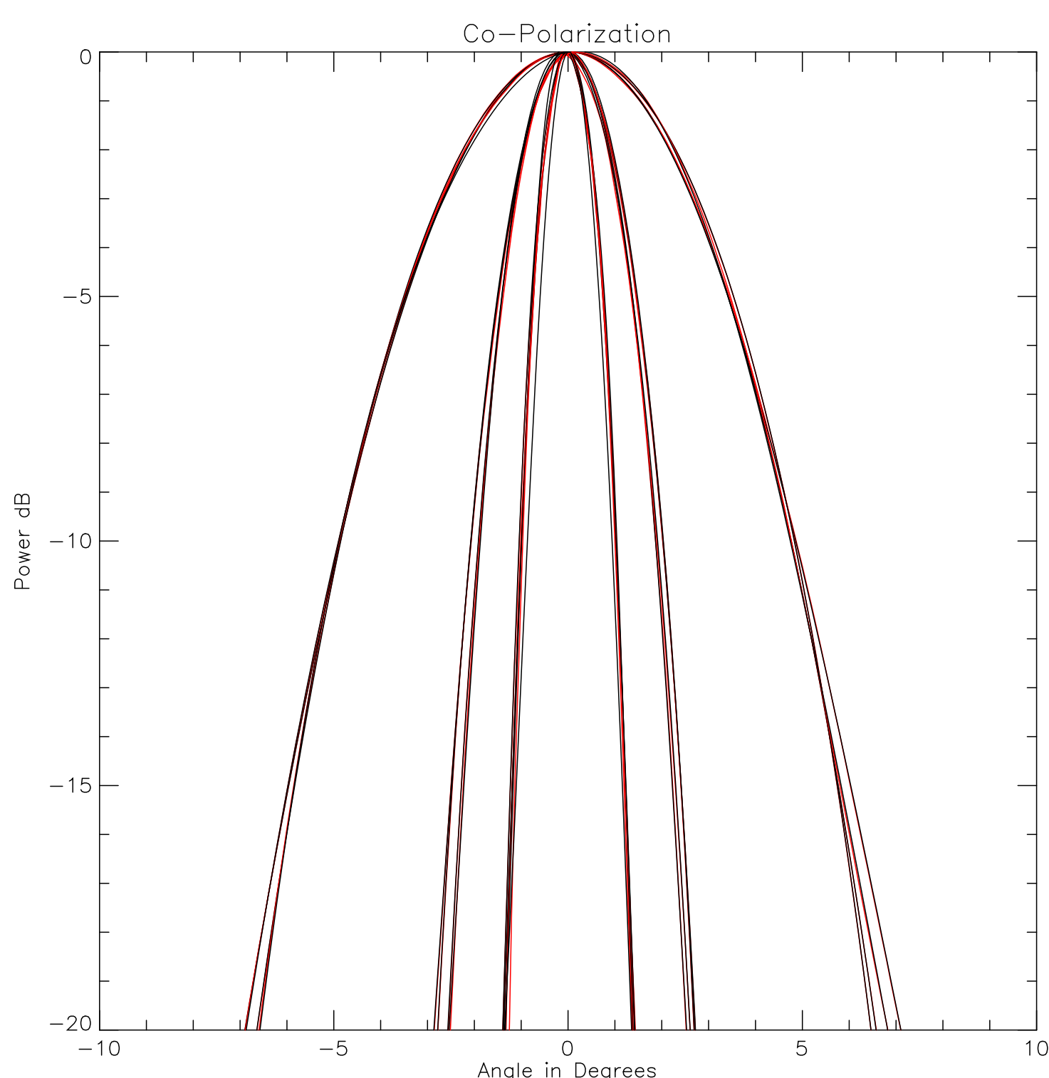
ATMS Antenna Patterns and Polynomial Fit
