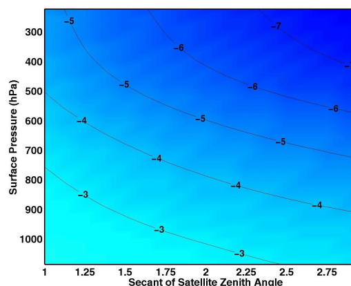
Fig 1: Comparison of the bias (K) across 52 atmospheres between BT(\langle \mathfrak{S}_s F^\dagger \rangle) and BT(\langle \mathfrak{S}_s \rangle \langle F^\dagger \rangle) for AIRS channel 1018.
