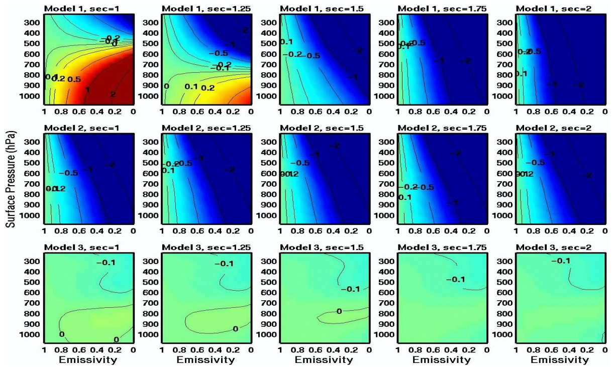
Fig 4: M1, M2 & M3 bias (K) as a function of surface emissivity, surface pressure and zenith angle secant for AIRS channel 1018 (1007.86 (cm -1 )).
