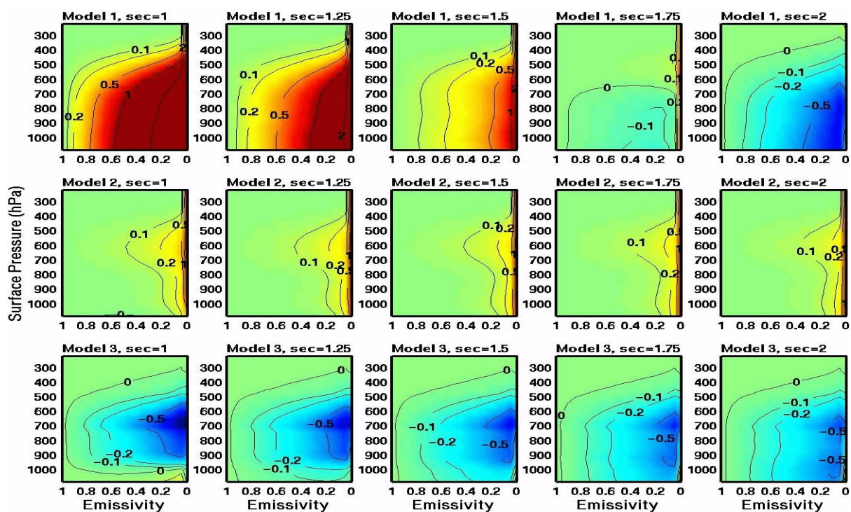
Fig 6: M1, M2 and M3 bias (K) as a function of surface emissivity, surface pressure and zenith angle secant for AIRS channel 610 (851.80 (cm -1 ))
