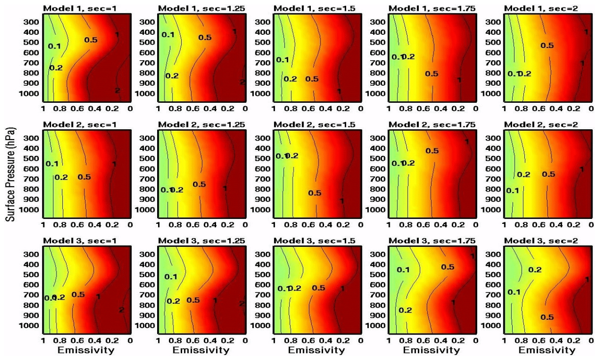
Fig 5: M1, M2 & M3 stdv (K) as a function of surface emissivity, surface pressure and zenith angle secant for AIRS channel 1018 (1007.86 (cm -1 )).
