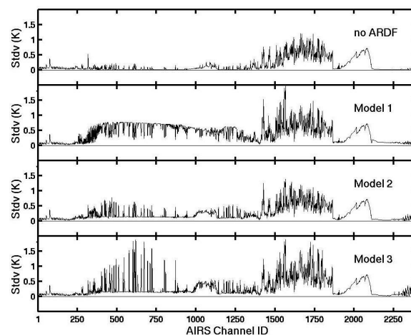
Fig 3: Stdv of the differences between the FLBL and the 3 FFMs for \epsilon=.7 and P_s=1013.25 hPa for a nadir view.
