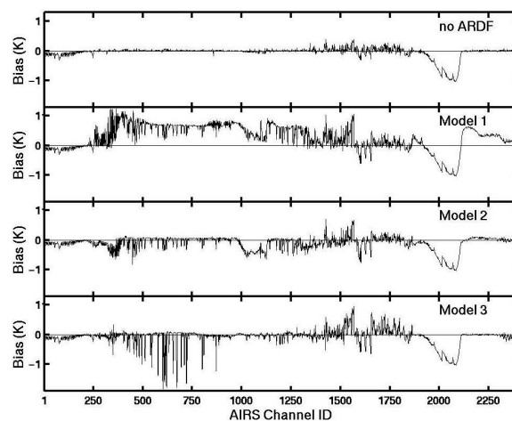
Fig 2: Bias of the differences between the FLBL and the 3 FFMs for \epsilon=.7 and P_s=1013.25 hPa for a nadir view.
