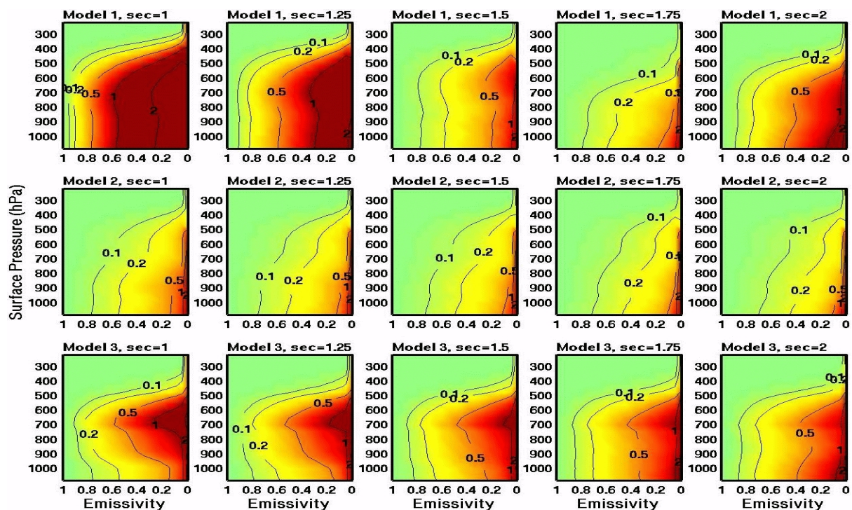
Fig 7: M1, M2 and M3 stdv (K) as a function of surface emissivity, surface pressure and zenith angle secant for AIRS channel 610 (851.80 (cm -1 )).
