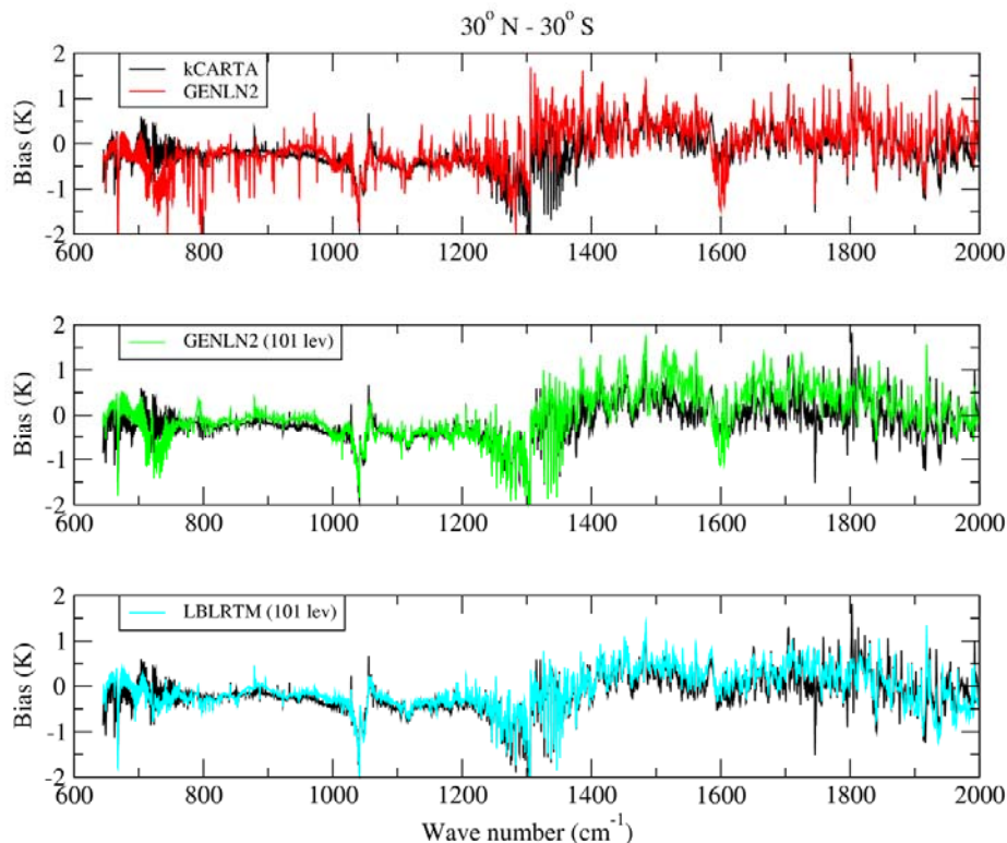
Figure 8: the mean value of the difference between observed and computed brightness temperatures for the tropics.
