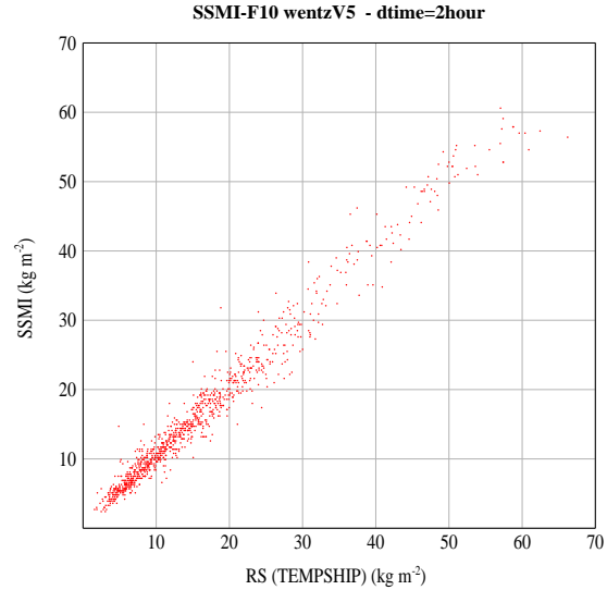
figure 2: SSMI TCWV as function as colocated ship radiosounding (2 hour time lag) between November and June 1997 ( \text{kg/m}^2 )
