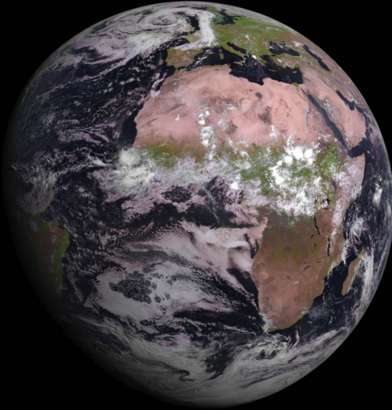
MSG-4 SEVIRI First Image 4 August 2015 10:00 UTC
