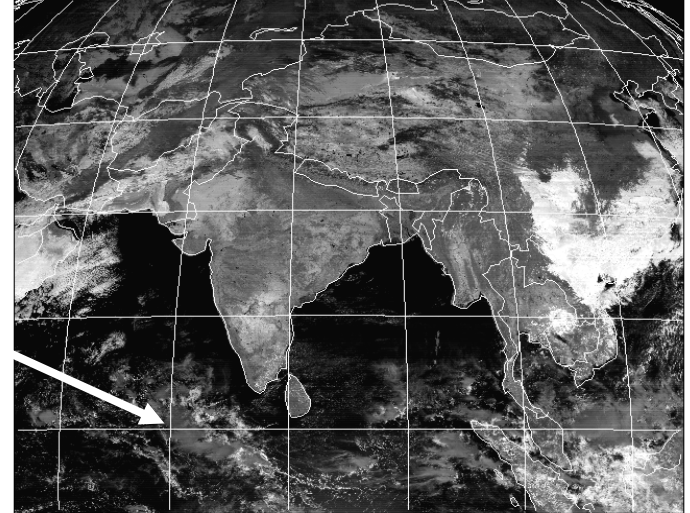
INSAT-2E SWIR (1.62um) 18-1-2000 11:30
